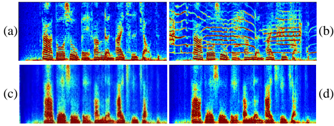
Fig. 4 Spectrograms: (a) clean speech, (b) noisy speech with 0dB SNR, (c) enhanced speech by A-DNN, and (d) enhanced speech by AV-DNN.
