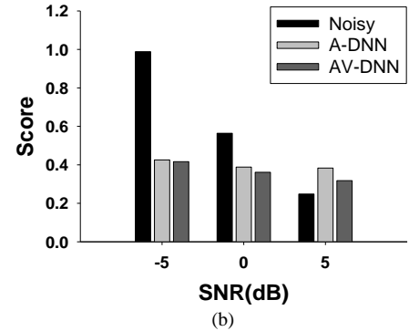
Fig. 5 Average scores of (a) SSNRI and (b) SDI. A-DNN and AV-DNN denote DNN using audio and audio-visual features, respectively.
