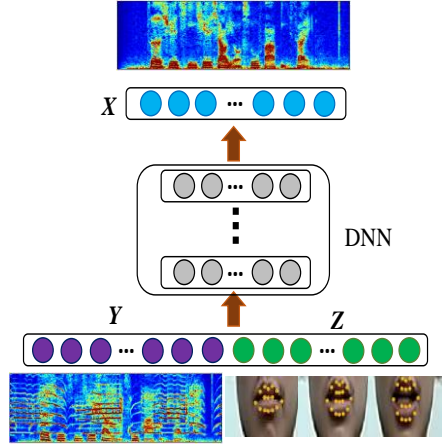
Fig. 2 Training audio-visual DNN neurons with pairs of noisy speech features concatenated with visual features and corresponding clean speech features.
