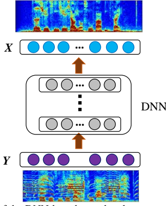
Fig. 1 Structure of the DNN-based speech enhancement approach.
